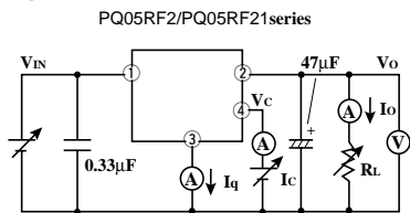
Fig.1 Test Circuit
