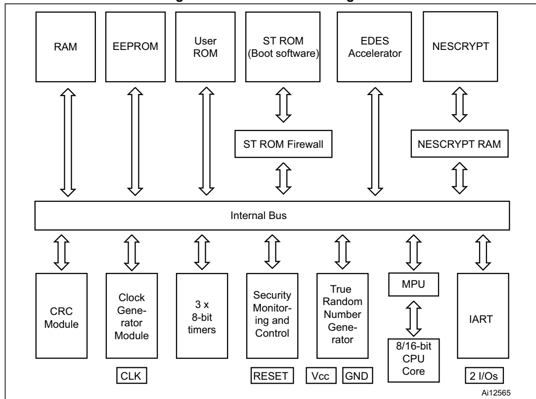
Figure 1. ST23YL18 block diagram
